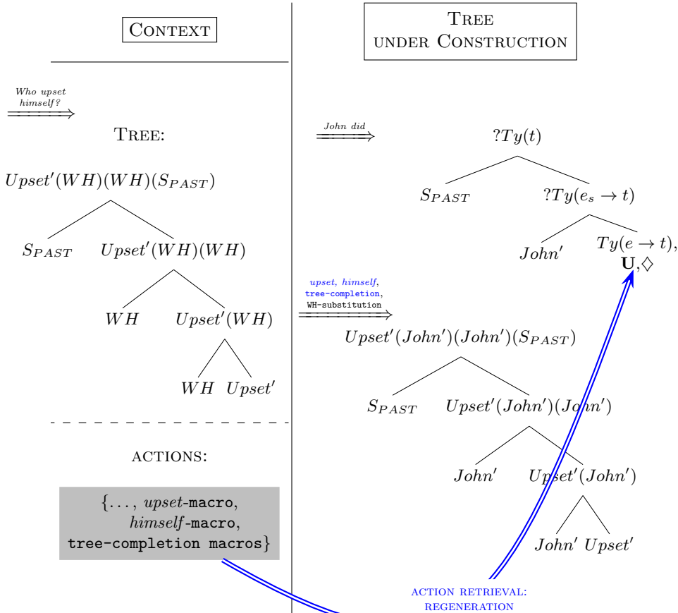
Figure 1.6. Action replay from context at the ellipsis site
