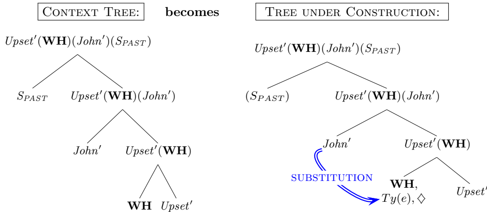
Figure 1.7. A short answer with binding restrictions
