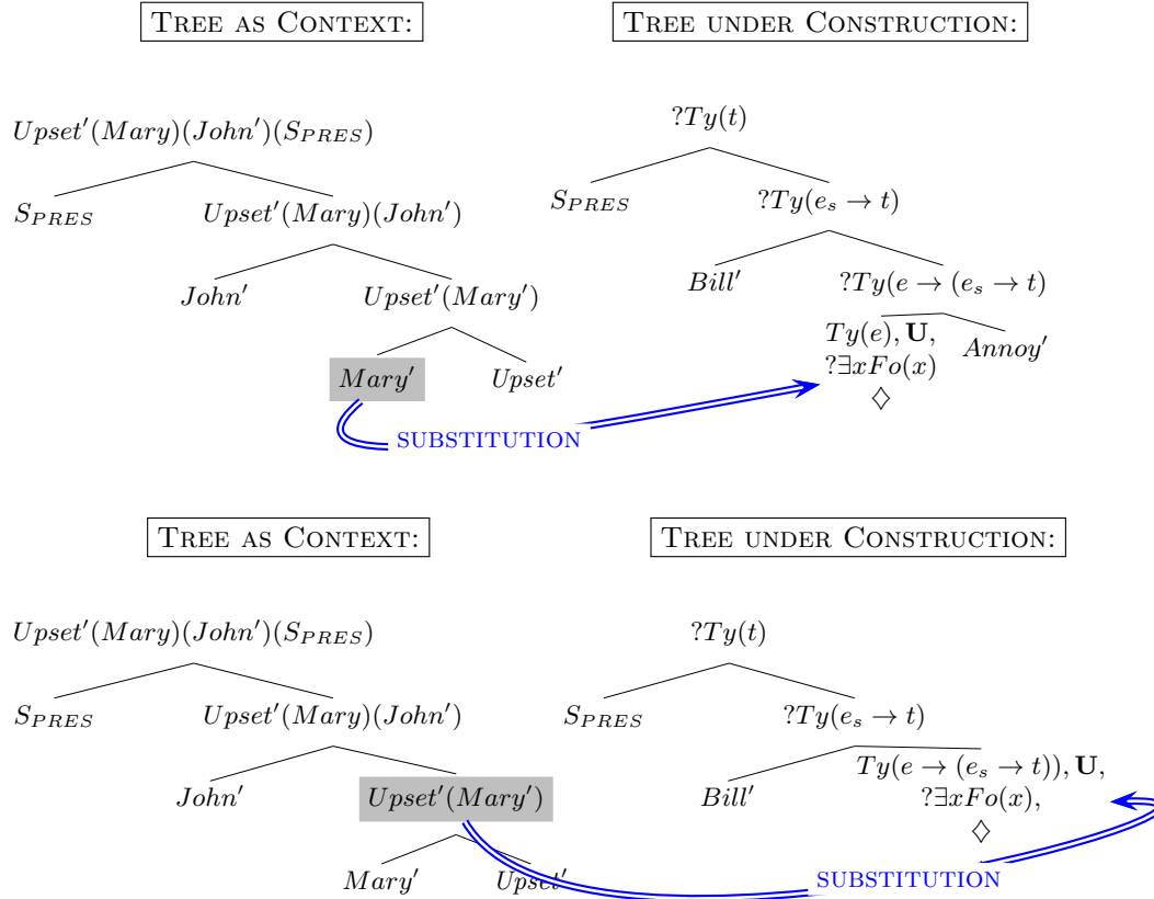
Figure 1.5. Substitution from context at the ellipsis site of (24): pronominal-anaphora (top) and VP-Ellipsis (bottom)
