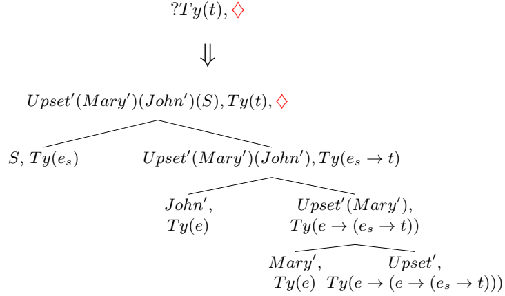
Figure 1.1. Processing John upset Mary in DS
