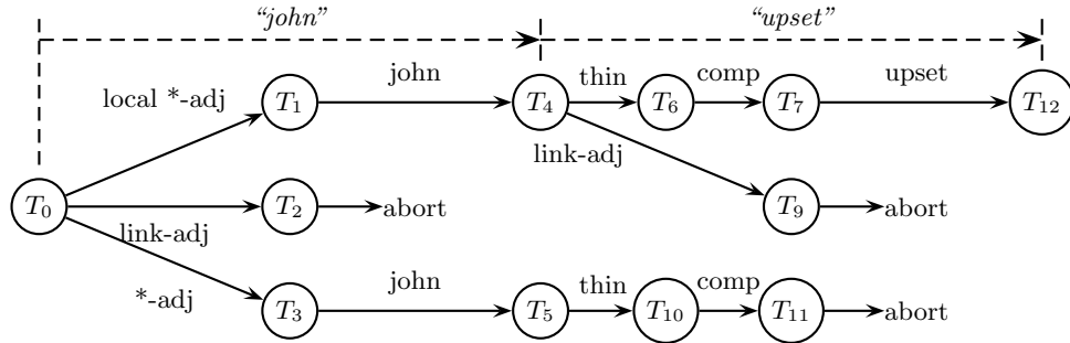
Figure 1.4. DS parsing context as a graph: actions (edges) are transitions between partial trees (nodes).
